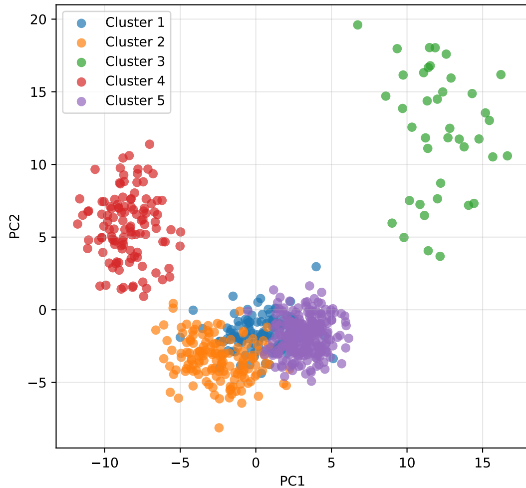
Predicted clusters (PCA + K-means)
